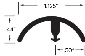
1.125" Snap Down T-Mold | 145VS
